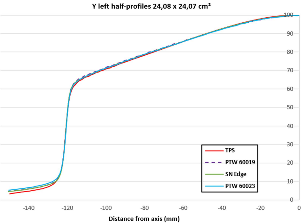
Fig. 7 Y left half-profiles comparison between the TPS and the high resolution detector measurements for a 24.08×24.07 cm 2 field size
